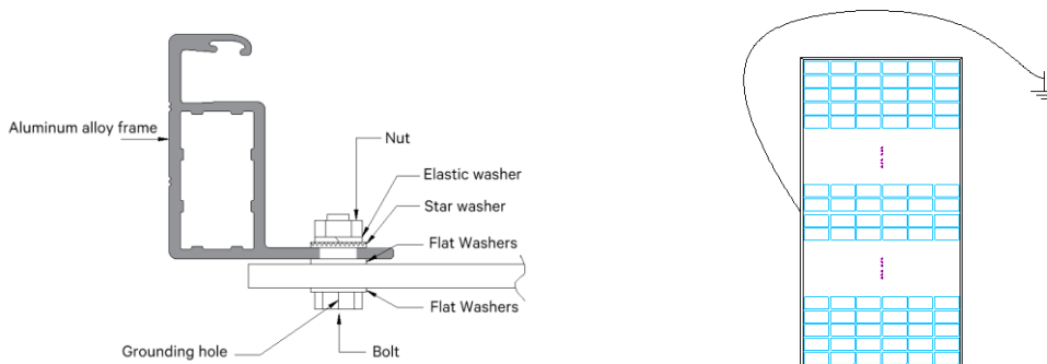
Figure 13-2: Grounding diagram
